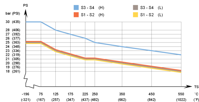
AlfaNova HP 27 - PED approved pressure/temperature graph
