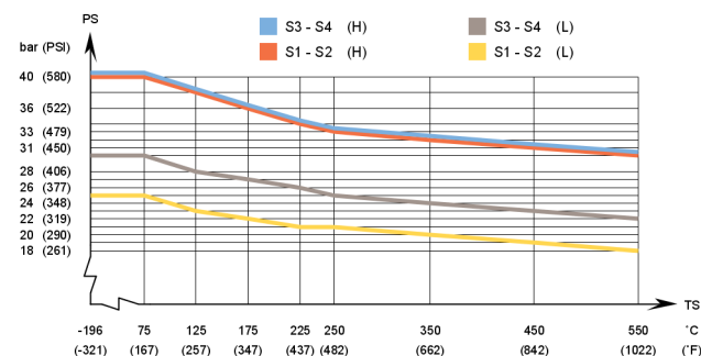
AlfaNova XP27 - PED approved pressure/temperature graph
