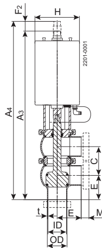
Change-over valve
