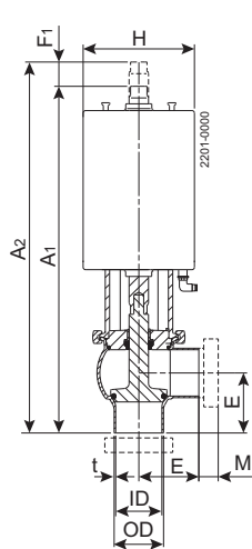
Shut-off valve
