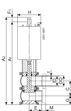
Shut-off valve
