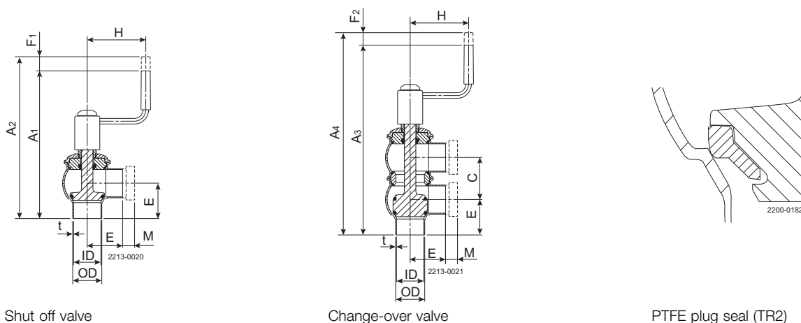
Fig. 2. Dimensions.
