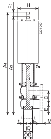
Change-over valve.
