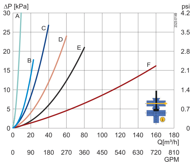
Figure 1. Pressure drop/capacity diagram, upper body
