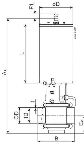
Figure 5. Unique Mixproof CIP Type 30
