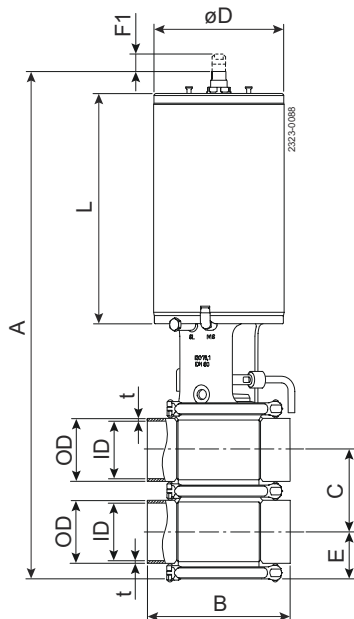
Figure 4. Unique Mixproof CIP
