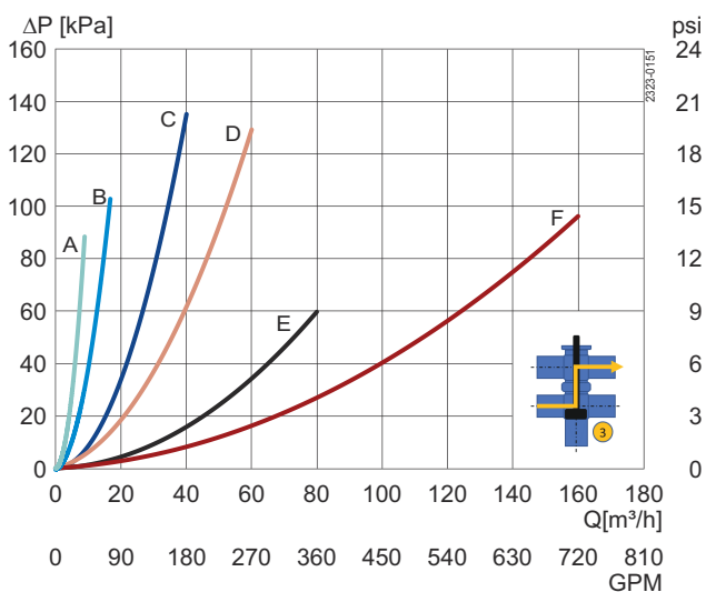
Figure 3. Pressure drop/capacity diagram, between bodies
