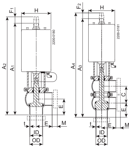
Shut-off valve
