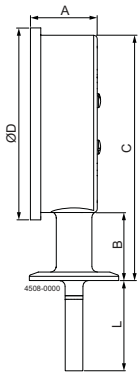
Clamp DN38 (ISO2852) / Clamp DN40 (DIN32676) TE67Dx1xxx1xxx
